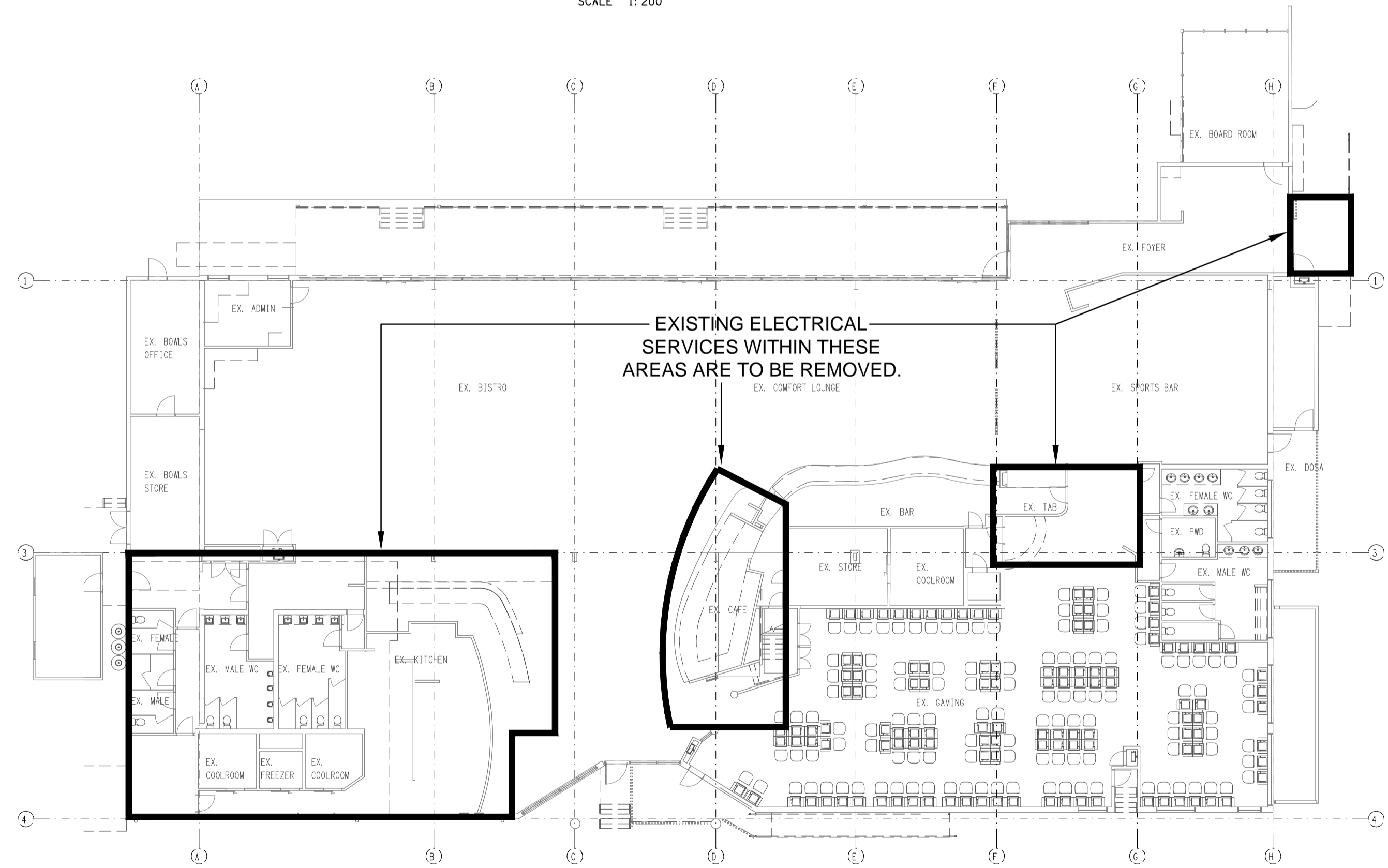
GROUND LEVEL DEMOLITION REFLECTED CEILING PLAN SCALE 1: 200
