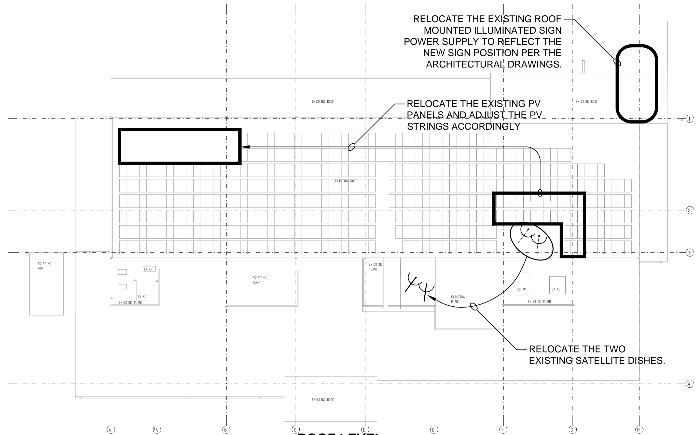
ROOF LEVEL RELOCATION PLAN SCALE 1: 200
