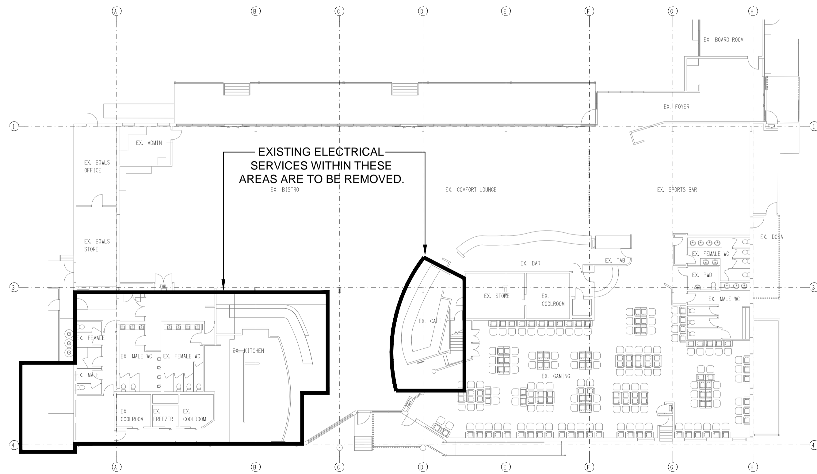
GROUND LEVEL DEMOLITION FLOOR PLAN SCALE 1: 200
